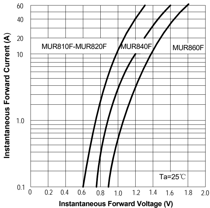
FIG3: Forward Voltage
